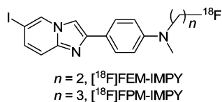
Figure 2. Structures of [ ^{18}\text{F} ]FEM-IMPY and [ ^{18}\text{F} ]FPM-IMPY.
