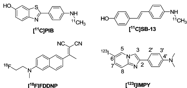
Figure 1. Four radioligands for imaging A \beta plaques in clinical research.
